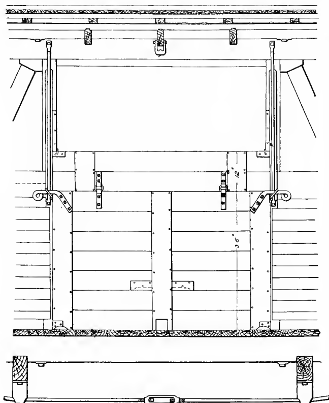
Fig. 1870. Interior Elevation.
